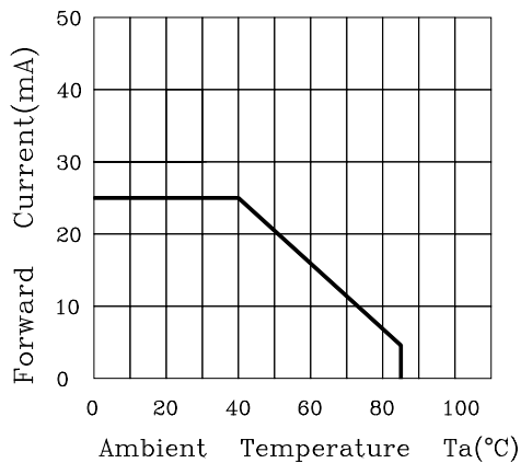
FORWARD CURRENT VS DERATING CURVE
